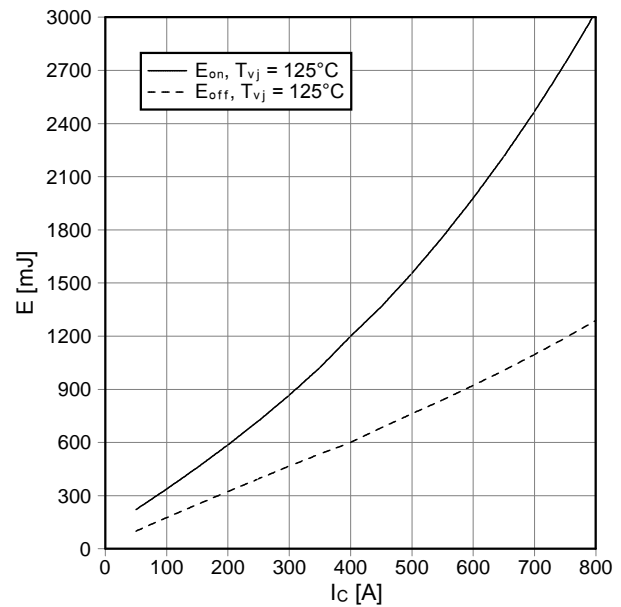
Schaltverluste IGBT-Wechselr. (typisch) switching losses IGBT-inverter (typical) E_{on} = f(I_c) , E_{off} = f(I_c) V_{GE} = \pm 15\text{ V} , R_{Gon} = 6,2\ \Omega , R_{Goff} = 13\ \Omega , V_{CE} = 1800\text{ V} , C_{GE} = 100\text{ nF}
