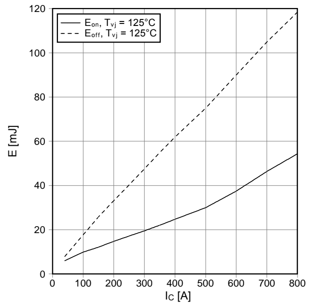
Schaltverluste IGBT-Brems-Chopper switching losses IGBT-brake-chopper E_{on} = f(I_c) , E_{off} = f(I_c) V_{GE} = \pm 15\text{ V} , R_{Gon} = 1.8\ \Omega , R_{Goff} = 1.8\ \Omega , V_{CE} = 600\text{ V}
