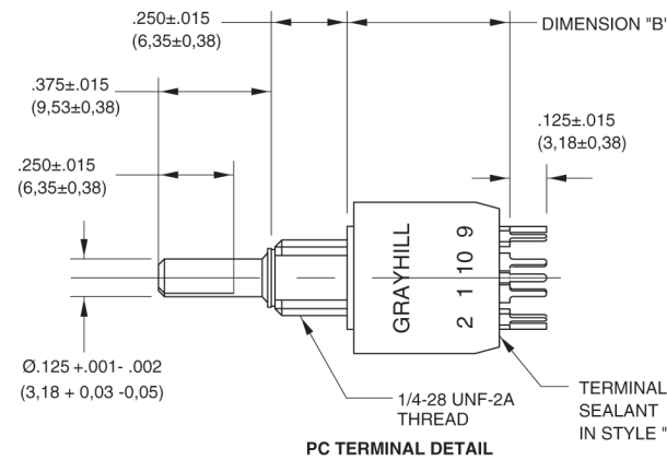
PC TERMINAL DETAIL All angles of throw, except 22.5°
