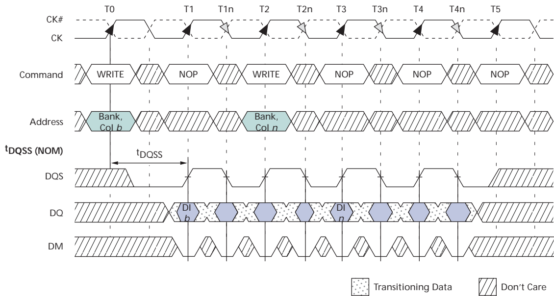
Figure 39: Consecutive WRITE-to-WRITE
