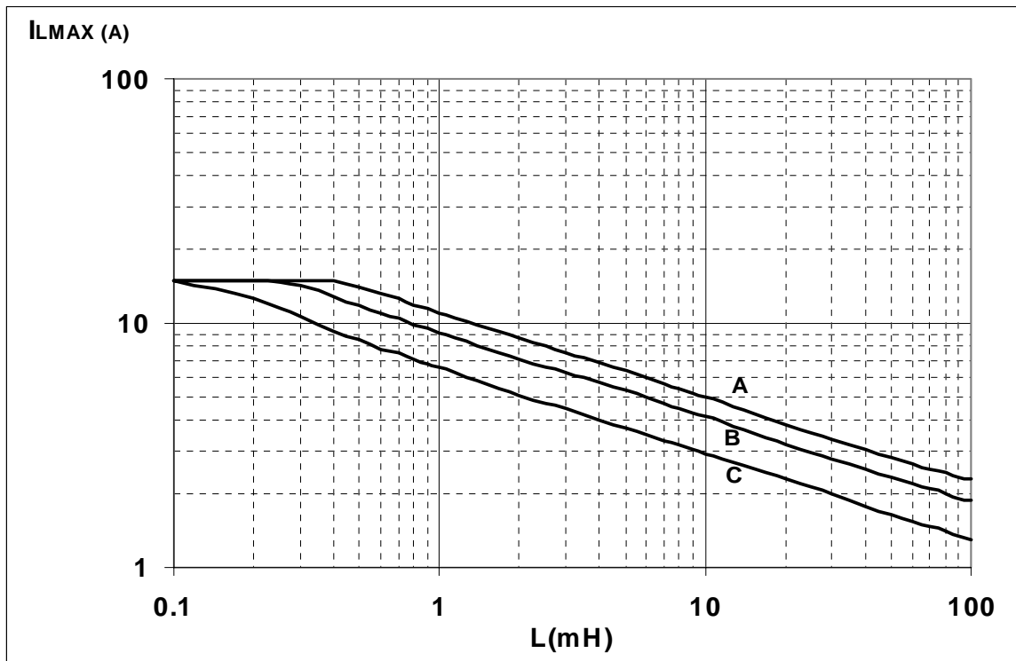
Figure 27. Maximum turn off current versus load inductance
