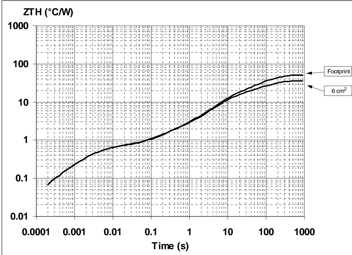
Figure 30. PowerSO-10 Thermal Impedance Junction Ambient Single Pulse
