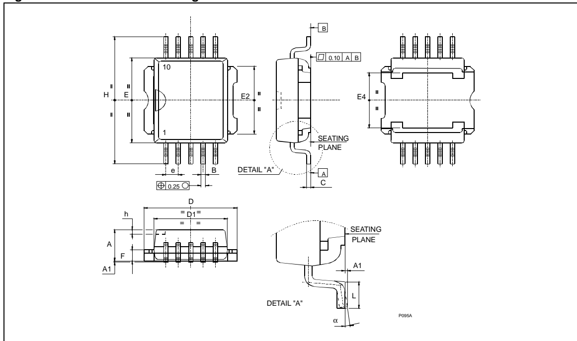
Figure 32. PowerSO-10™ Package Dimensions
