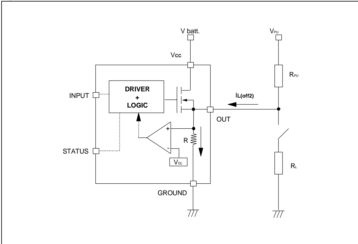
Figure 9. Open Load detection in off state
