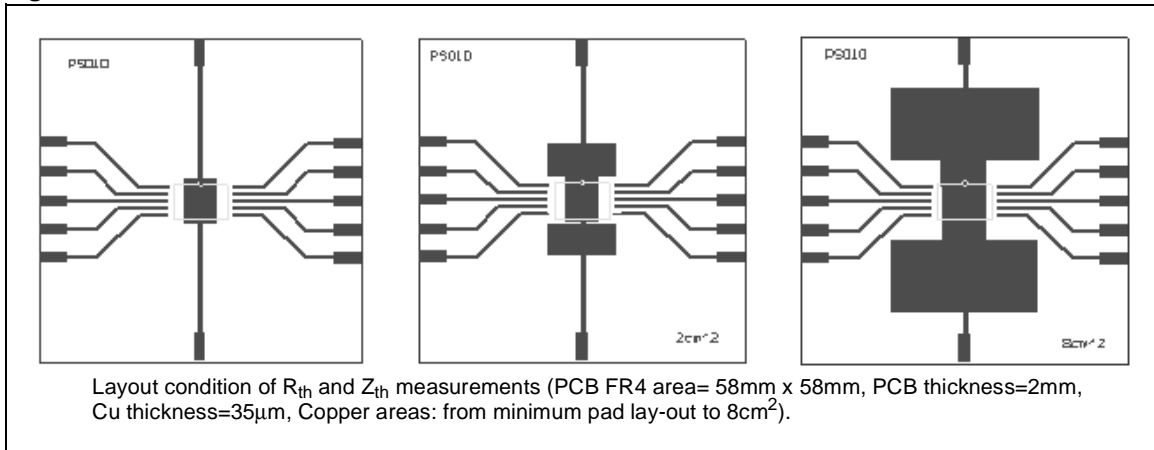
Figure 28. PowerSO-10™ PC Board
