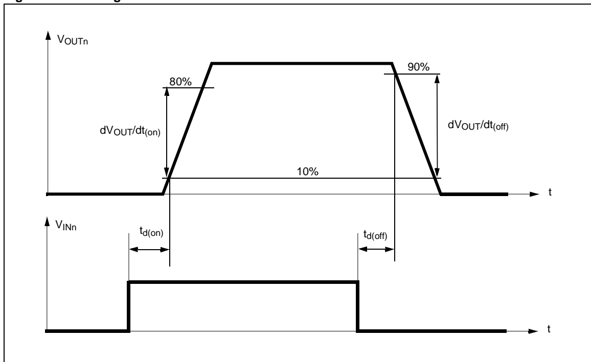
Figure 6. Switching Time Waveforms
