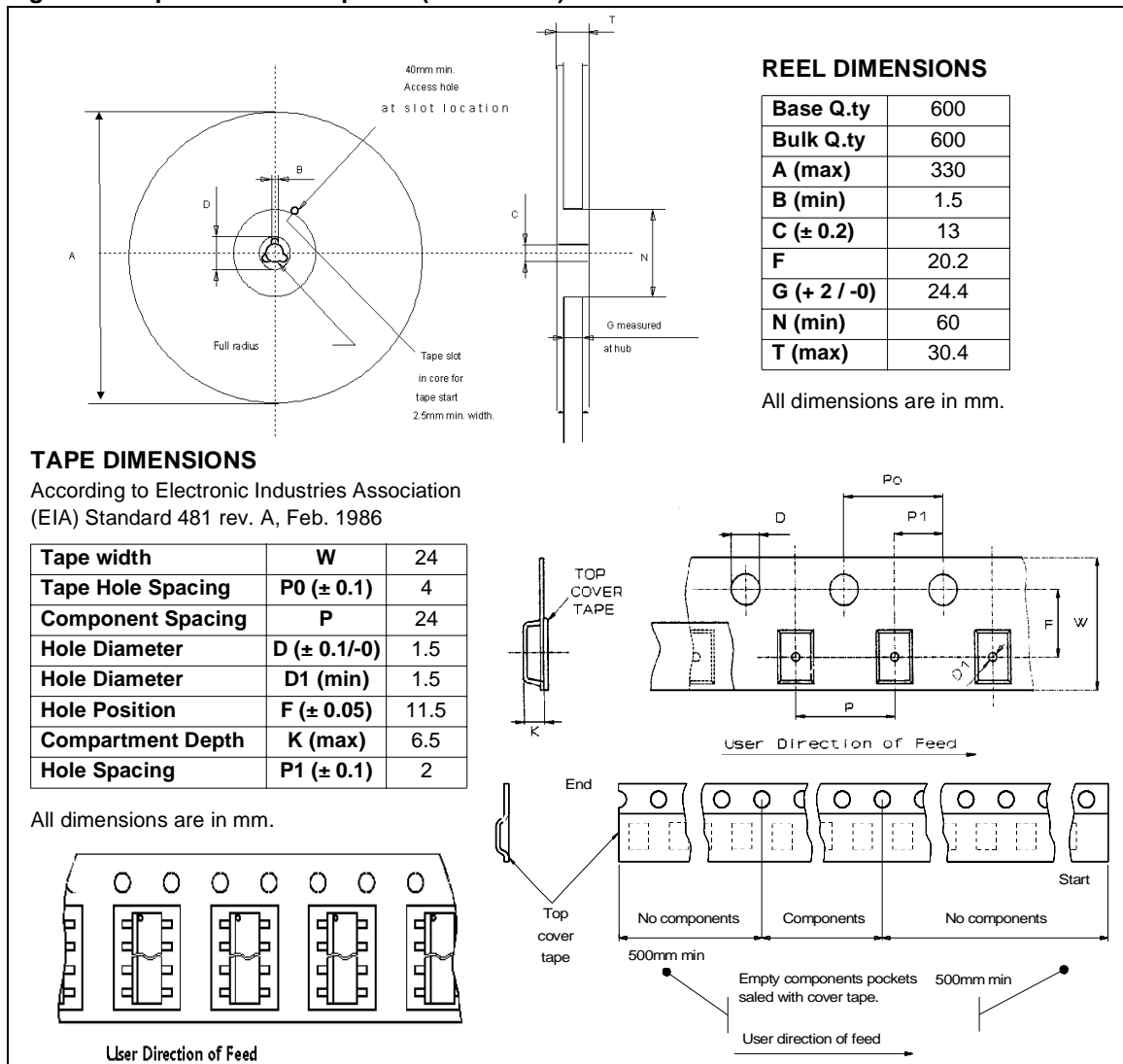
Figure 34. Tape And Reel Shipment (suffix “TR”)
