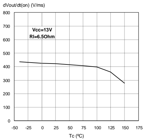
Figure 23. Turn-on Voltage Slope
