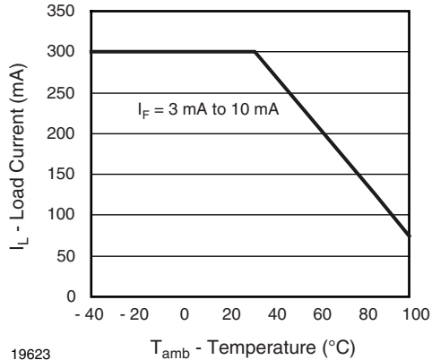
Fig. 1 - Recommended Operating Condition
