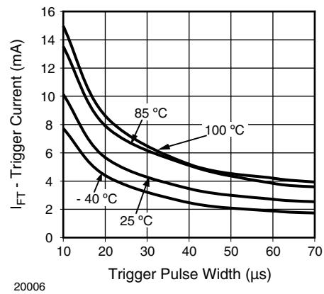
Fig. 1 I_{FT} vs. LED Pulse Width
