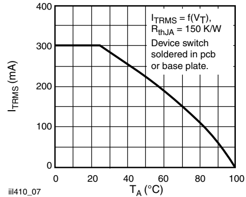
Fig. 5 - Current Reduction
