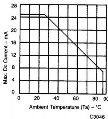
Fig. 4. Maximum Forward Allowable DC Current Per Segment vs. of Ambient Temperature
