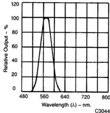
Fig. 2. Spectral Response
