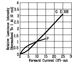
Fig3. RELATIVE LUMINOUS INTENSITY VS. FORWARD CURRENT
