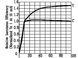
Fig7. RELATIVE LUMINOUS EFFICIENCY (LUMINOUS INTENSITY PER UNIT CURRENT) VS. PEAK CURRENT
