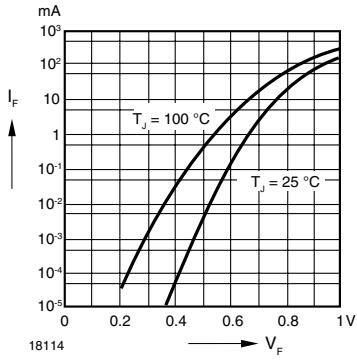
Figure 1. Forward characteristics
