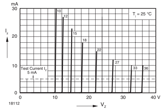
Figure 17. Breakdown Characteristics
