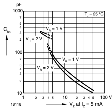
Figure 5. Capacitance vs. Zener Voltage
