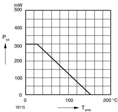
Figure 2. Admissible Power Dissipation vs. Ambient Temperature
