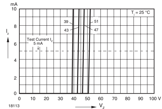
Figure 18. Breakdown Characteristics
