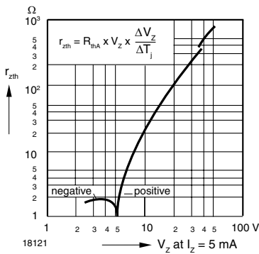
Figure 8. Thermal Differential Resistance vs. Zener Voltage
