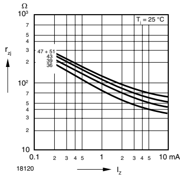
Figure 7. Dynamic Resistance vs. Zener Current
