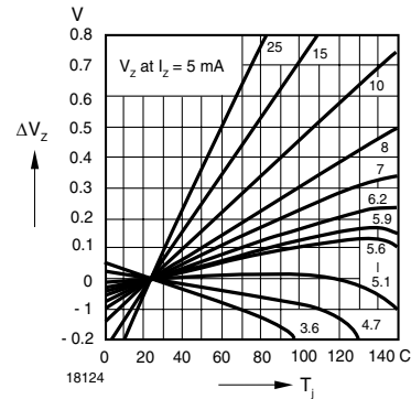
Figure 11. Change of Zener Voltage vs. Junction Temperature
