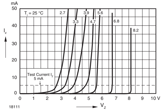
Figure 16. Breakdown Characteristics
