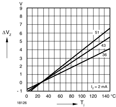
Figure 13. Change of Zener Voltage vs. Junction Temperature
