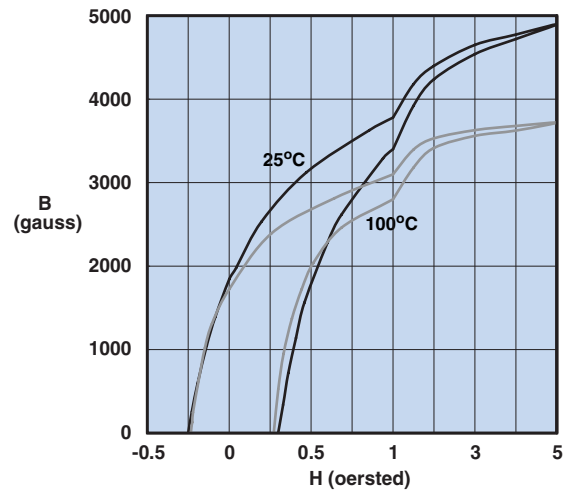
Measured on an 18/10/6mm toroid at 10kHz.
