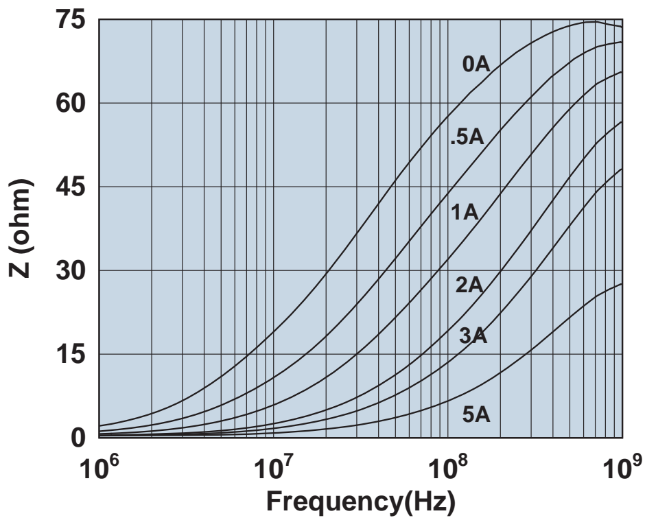
Impedance vs. frequency with dc bias.
