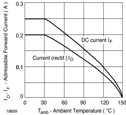
Figure 2. Admissible Forward Current vs. Ambient Temperature
