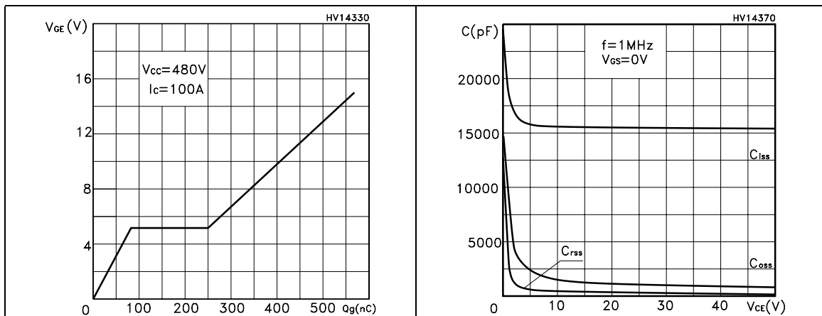
Figure 5. Gate charge vs gate-source voltage
