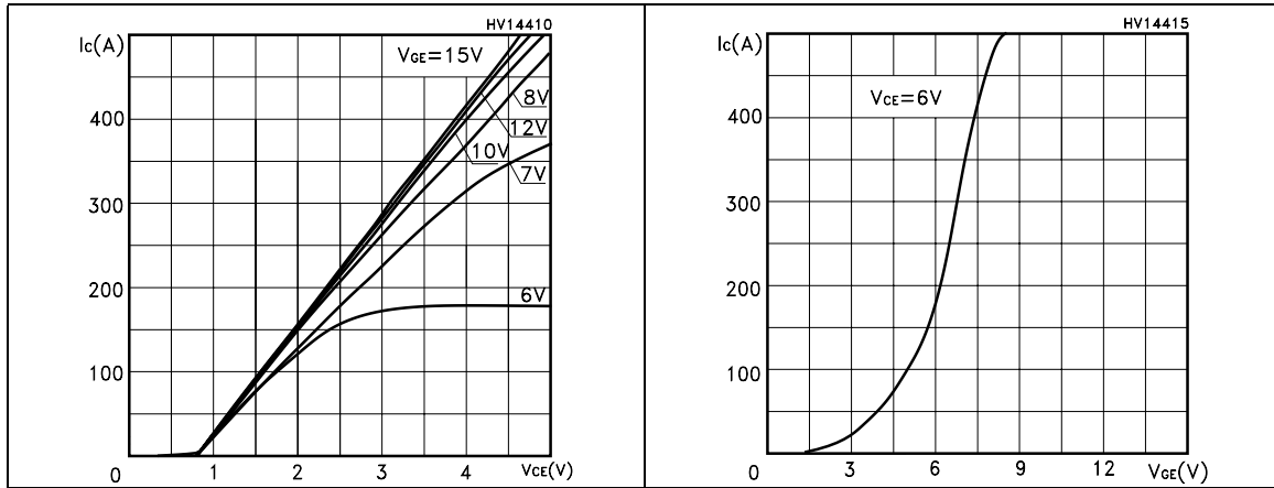
Figure 3. Transconductance
