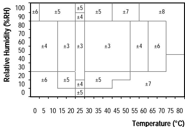
Figure 5 Maximal tolerance of relative humidity measurements given in %RH for temperatures 0 – 80°C.
