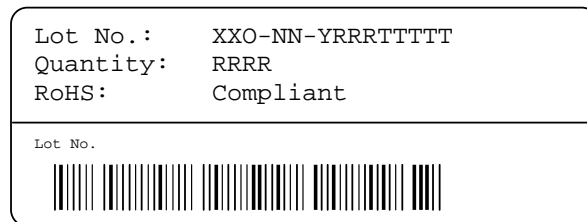
Figure 12: First label on reel: XX = Sensor Type (21 for SHT21), O = Output mode (D = Digital, P = PWM, S = SDM), NN = Chip Version, Y = last digit of year, RRR = number of sensors on reel divided by 10 (200 for 2000 units), TTTTT = Traceability Code.
