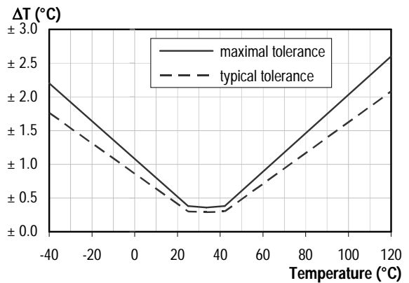
Figure 3 Maximal temperature accuracy tolerance
