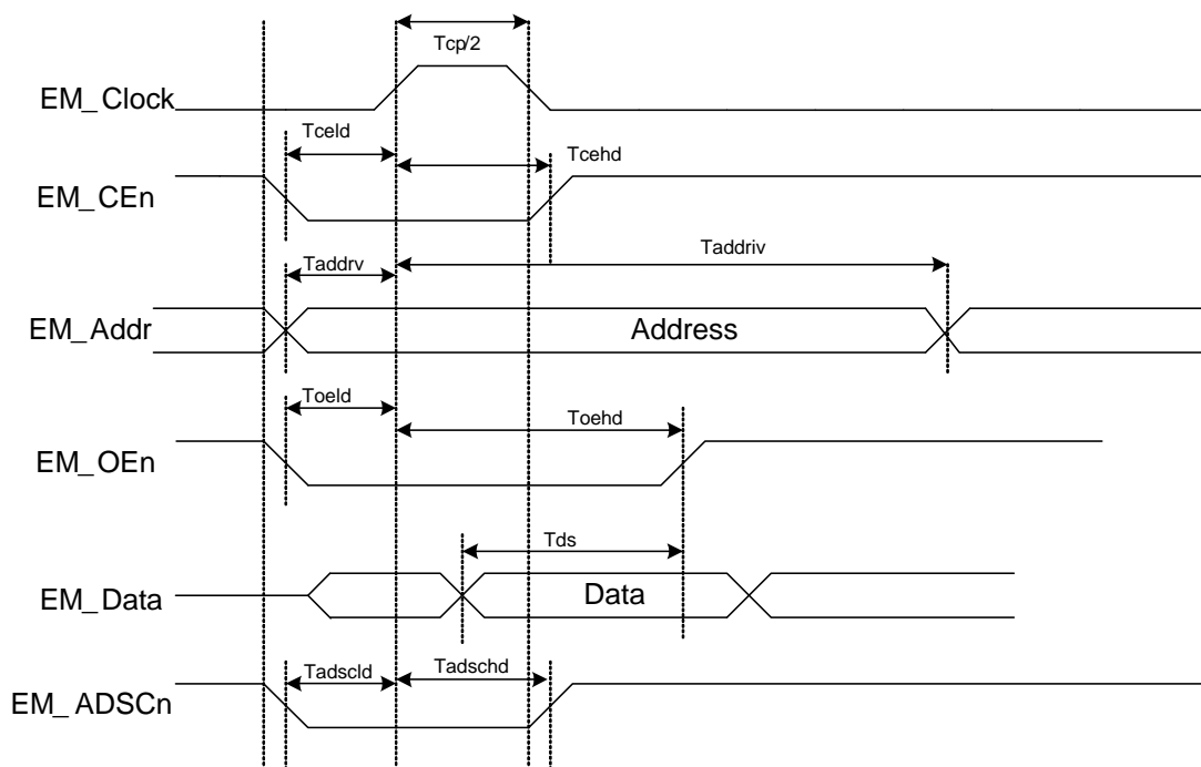
Figure 11-30. Synchronous Read Cycle Timing
