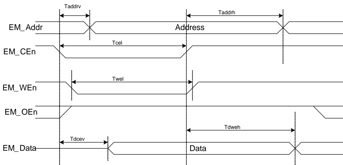
Figure 11-29. Asynchronous Write Cycle Timing
