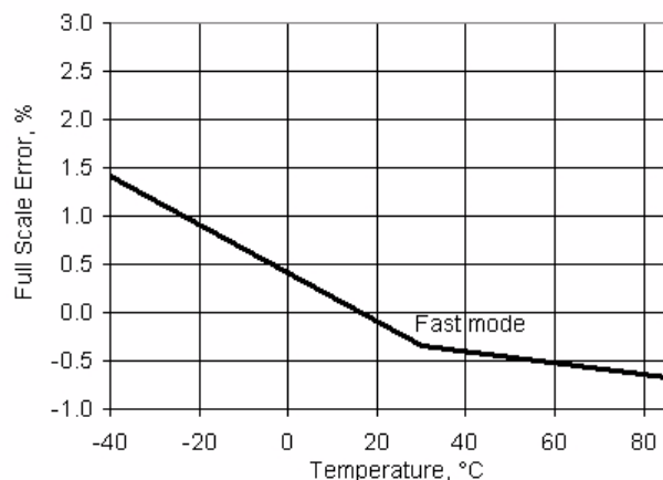
Figure 11-11. IDAC Full Scale Error vs Temperature, Range = 255 \mu A, Source Mode
