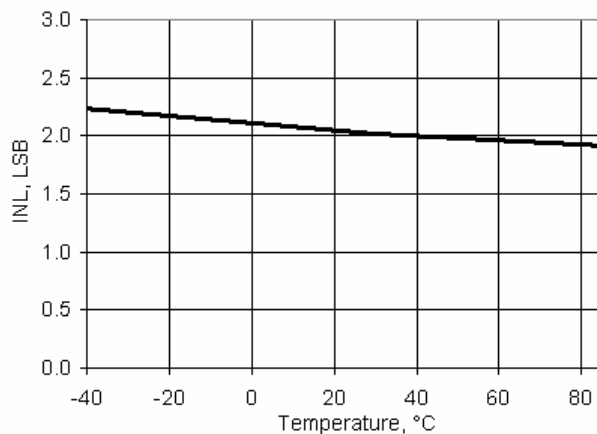
Figure 11-17. VDAC INL vs Temperature, 1 V Mode
