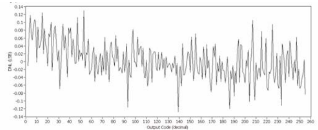
Figure 11-16. VDAC DNL vs Input Code, 1 V Mode
