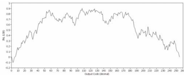
Figure 11-15. VDAC INL vs Input Code, 1 V Mode
