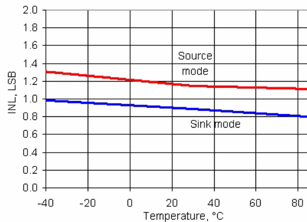
Figure 11-9. IDAC INL vs Temperature, Range = 255 \mu A, Fast Mode
