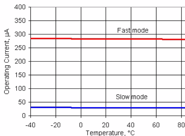
Figure 11-14. IDAC Operating Current vs Temperature, Range = 255 \mu A, Code = 0, Sink Mode
