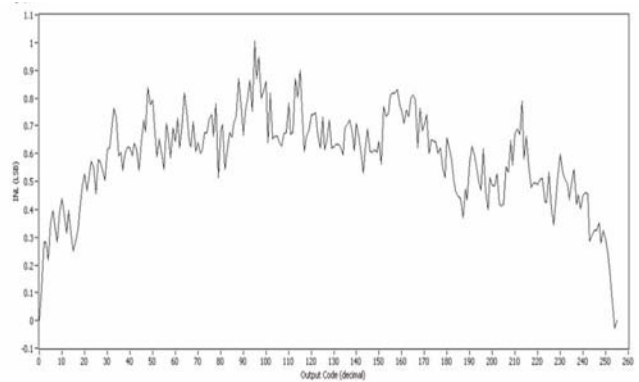
Figure 11-6. IDAC INL vs Input Code, Range = 255 \mu A, Sink Mode
