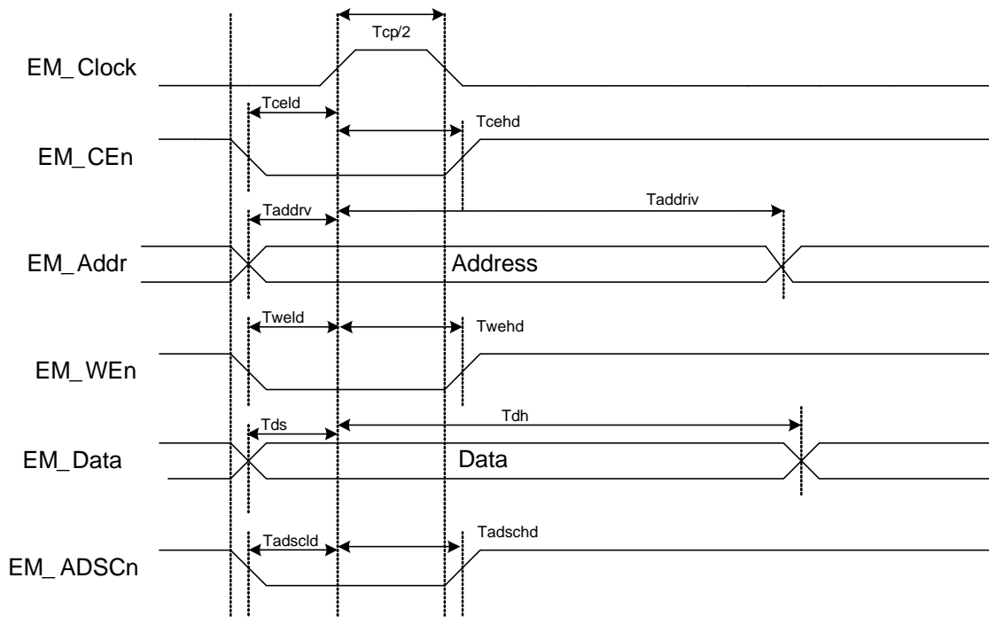
Figure 11-31. Synchronous Write Cycle Timing
