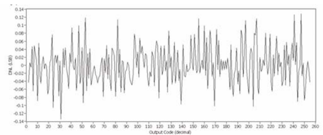
Figure 11-8. IDAC DNL vs Input Code, Range = 255 \mu A, Sink Mode
