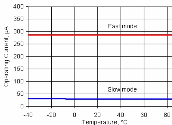
Figure 11-13. IDAC Operating Current vs Temperature, Range = 255 \mu A, Code = 0, Source Mode
