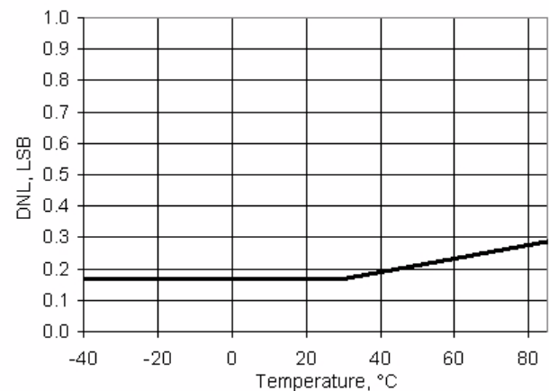
Figure 11-18. VDAC DNL vs Temperature, 1 V Mode
