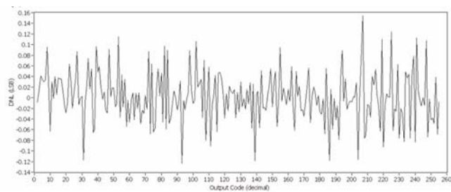
Figure 11-7. IDAC DNL vs Input Code, Range = 255 \mu A, Source Mode
