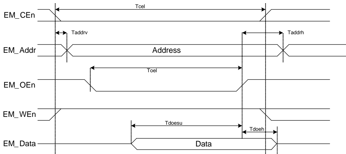
Figure 11-28. Asynchronous Read Cycle Timing
