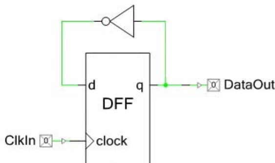
Figure 11-27. Clock to Output Performance
