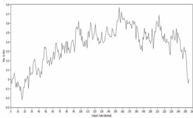
Figure 11-5. IDAC INL vs Input Code, Range = 255 \mu A, Source Mode
