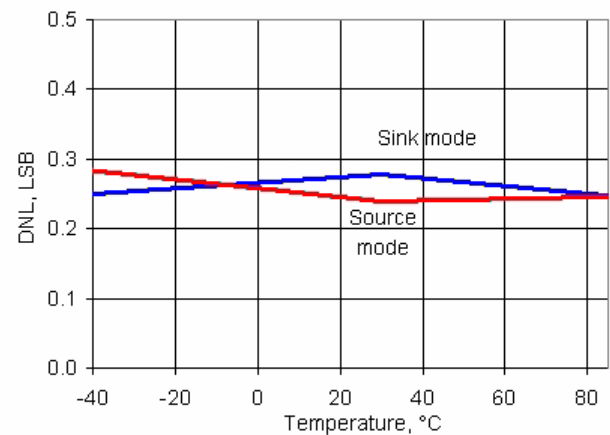
Figure 11-10. IDAC DNL vs Temperature, Range = 255 \mu A, Fast Mode
