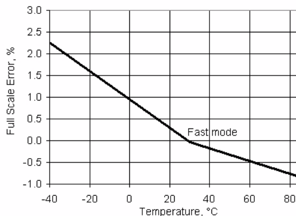
Figure 11-12. IDAC Full Scale Error vs Temperature, Range = 255 \mu A, Sink Mode
