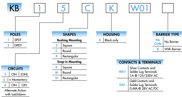
DESCRIPTION FOR TYPICAL ORDERING EXAMPLE KB15CKW01-12-FF
