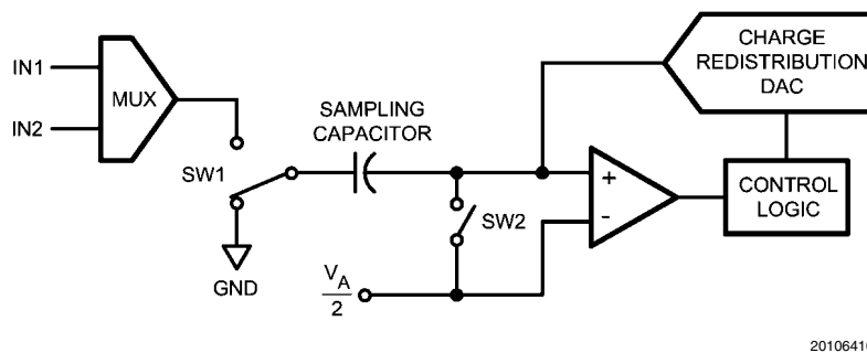
FIGURE 2. ADC122S051 in Hold Mode
