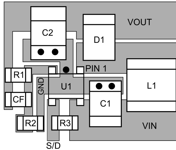
Recommended PCB Component Layout
