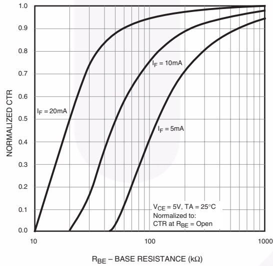
Fig. 9 CTR vs. R_{BE} (Unsaturated)
