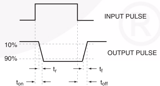
Figure 10. Switching Time Test Circuit and Waveforms
