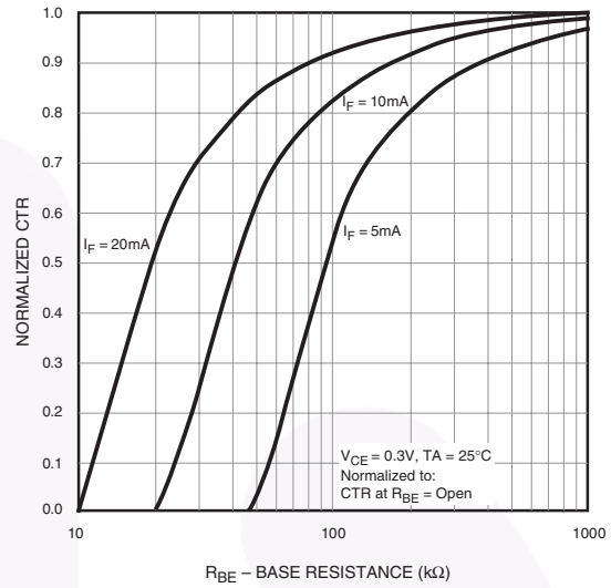
Fig. 8 CTR vs. R_{BE} (Saturated)
