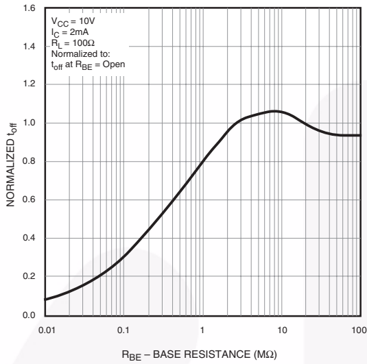
Fig. 7 Normalized t_{off} vs. R_{BE}
