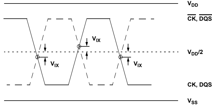
Figure 4. V_{IX} Definition
