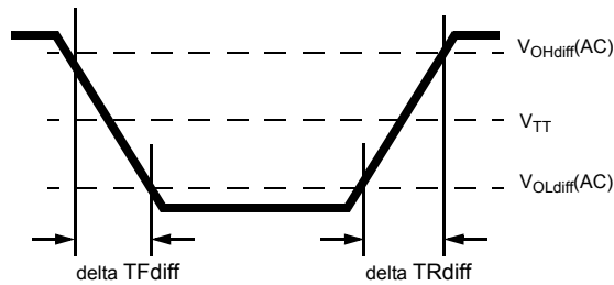
Figure 7. Differential output slew rate definition
