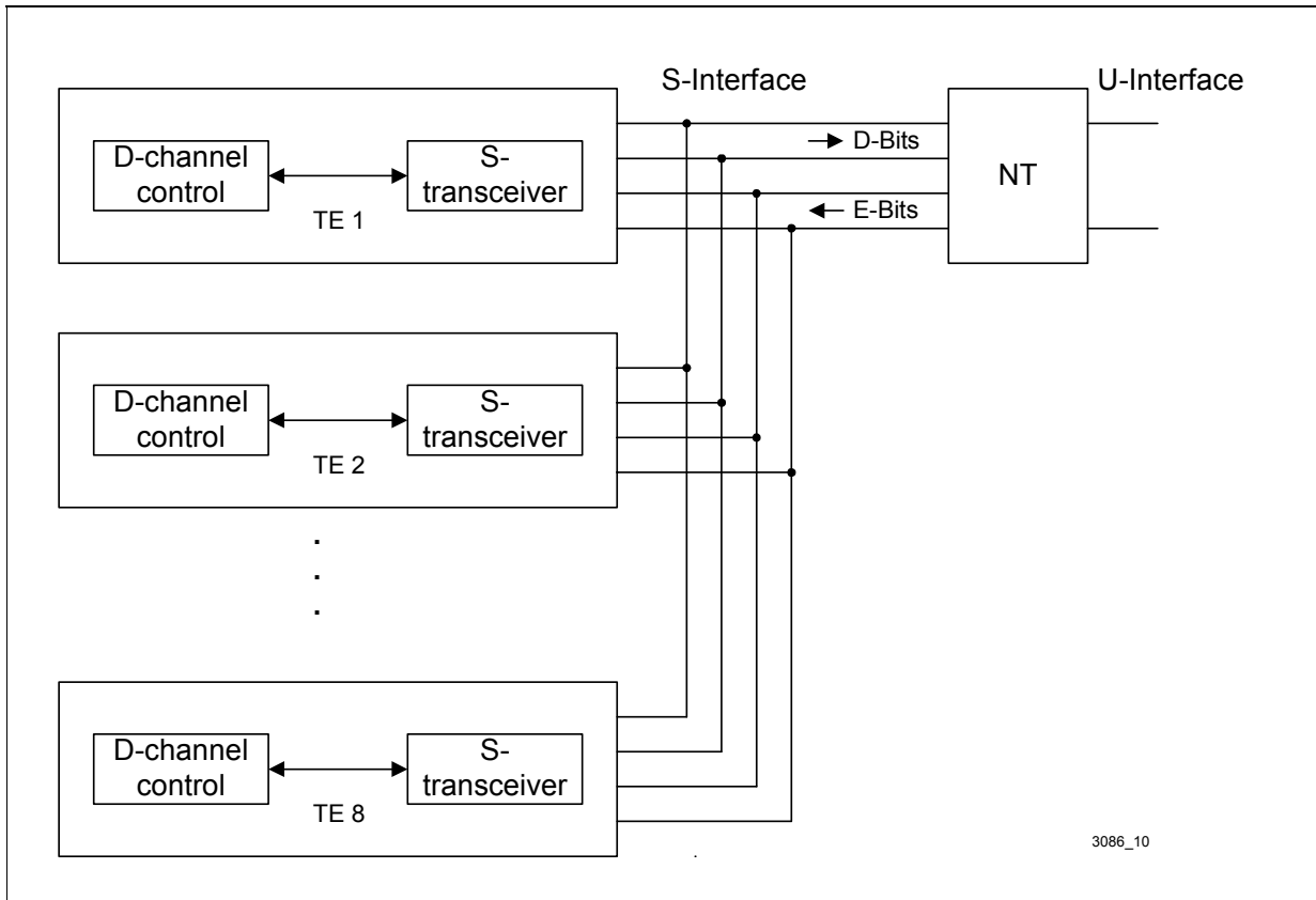
Figure 68 D-Channel Access Control on the S-Interface
