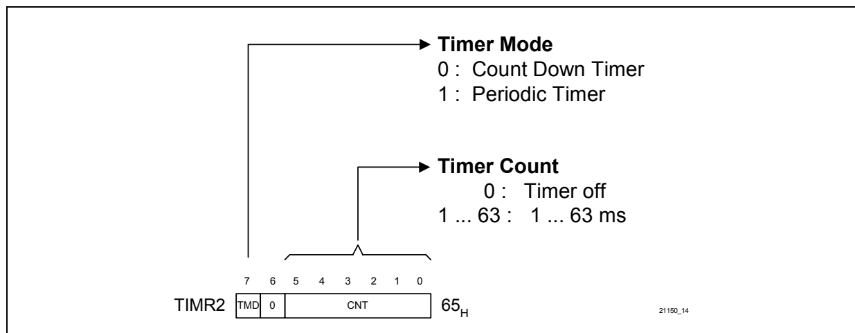
Figure 12 Timer 2 Register
