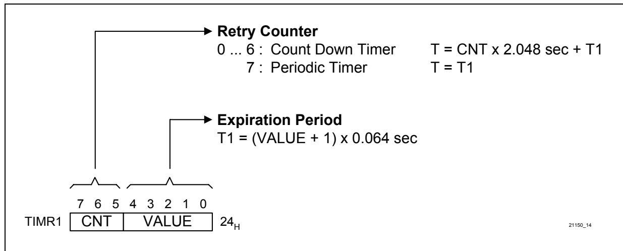
Figure 11 Timer 1 Register
