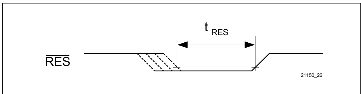
Figure 96 Reset Signal \overline{RES}
