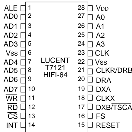
Figure 2. Pin Diagram
