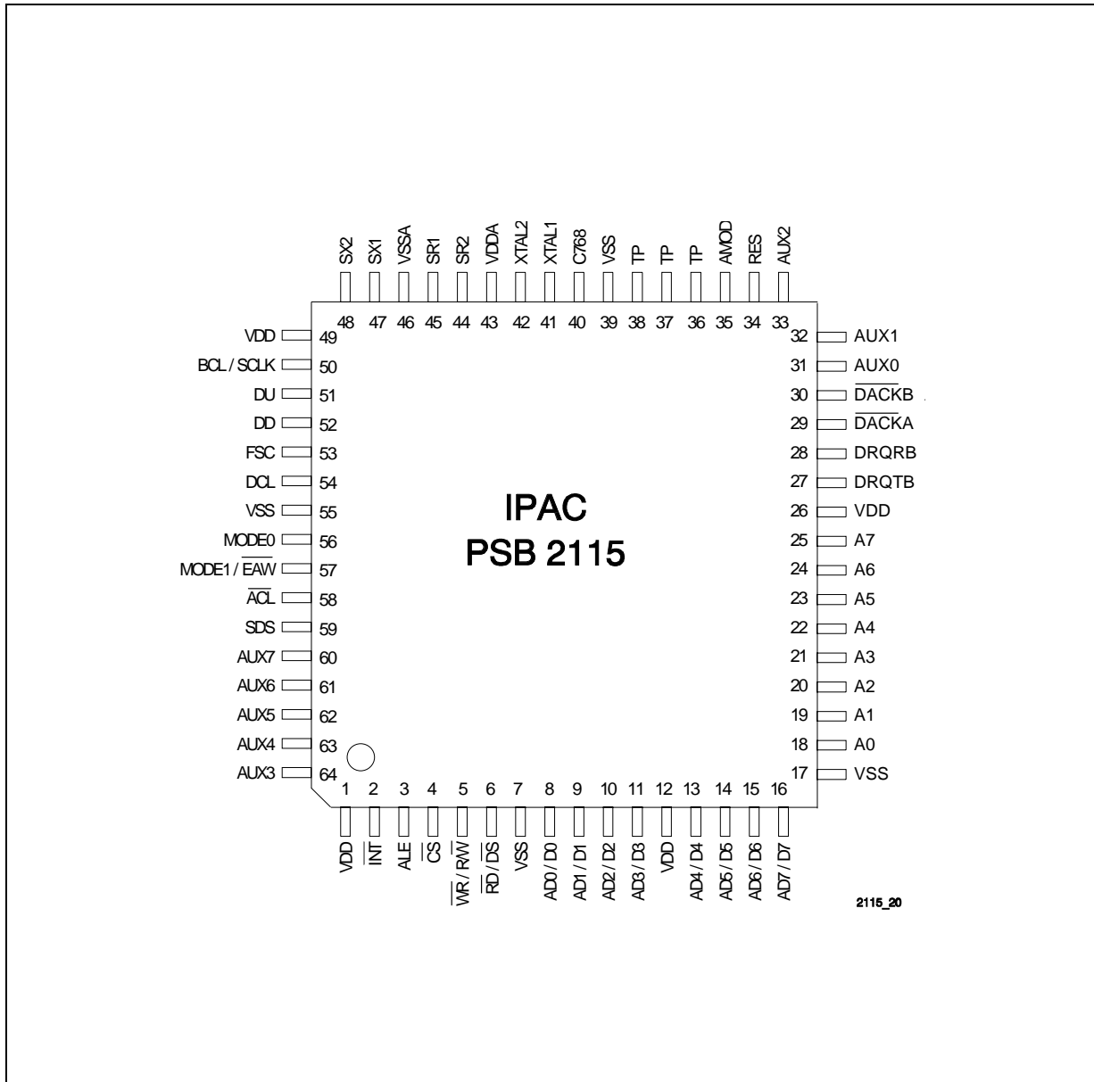
Figure 2 Pin Configuration
