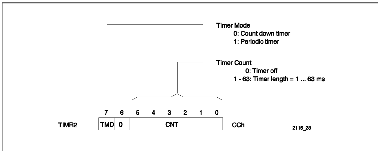
Figure 49 Timer 2 Register
