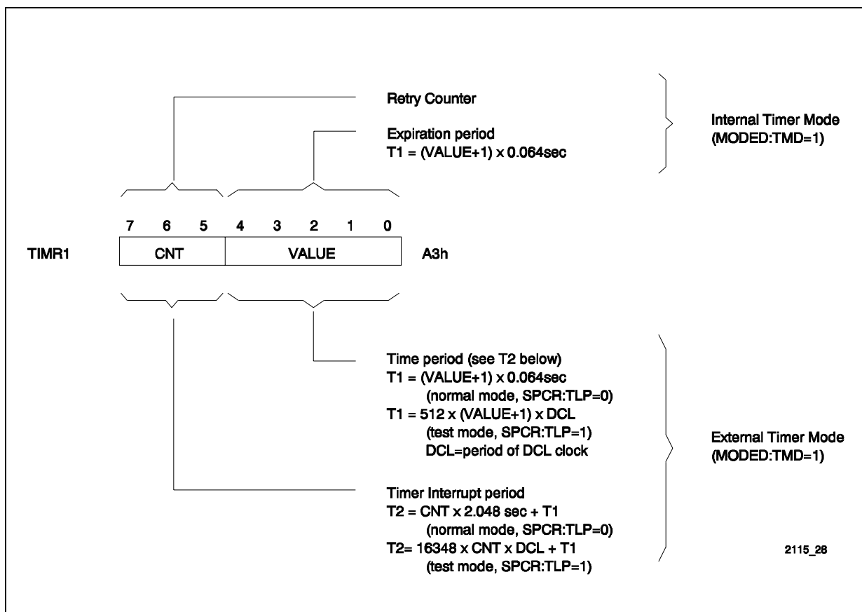
Figure 48 Timer 1 Register
