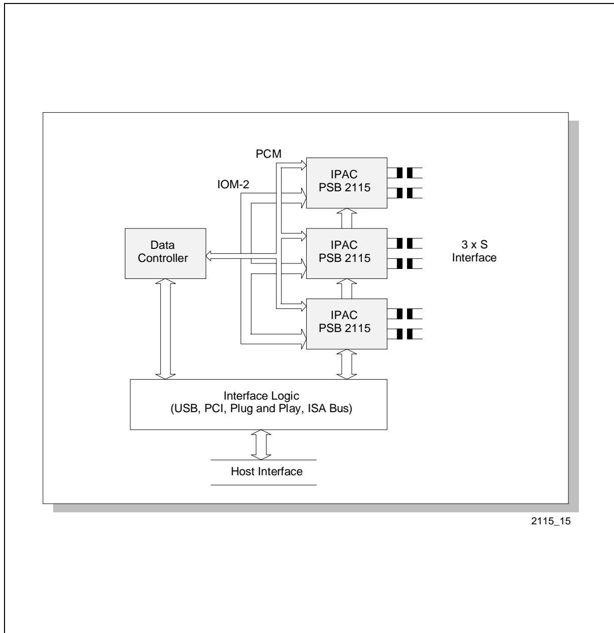
Figure 8 Multiline PC-Adapter
