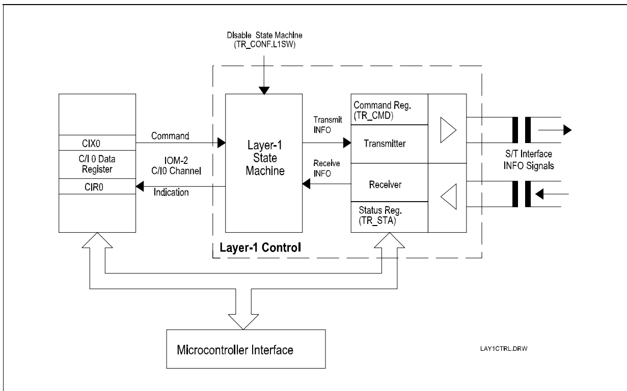
Figure 37 Layer-1 Control
