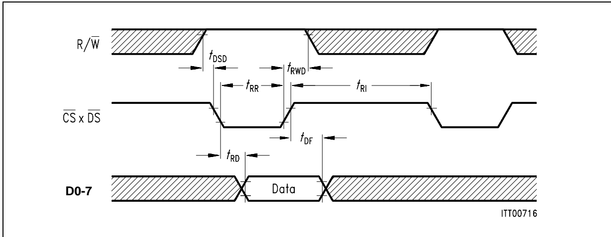
Figure 92 Microprocessor Read Timing
