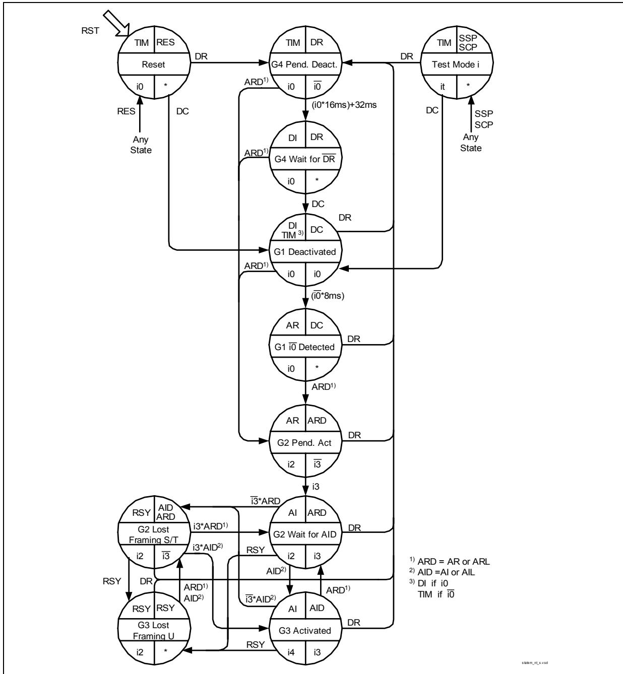
Figure 42 State Transition Diagram (NT)
