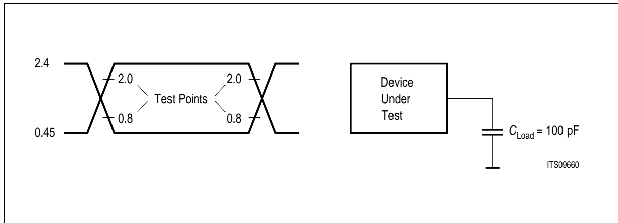
Figure 83 Input/Output Waveform for AC Tests
