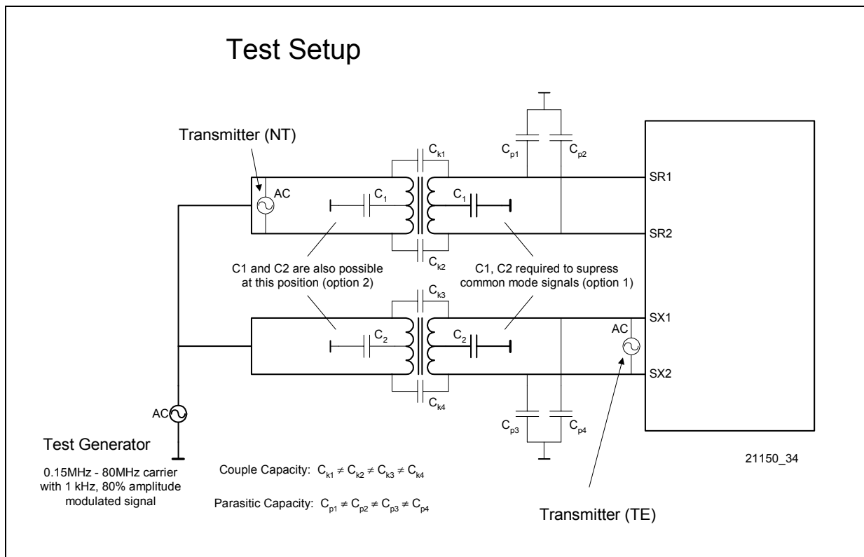
Figure 98 Transformer Circuitry
