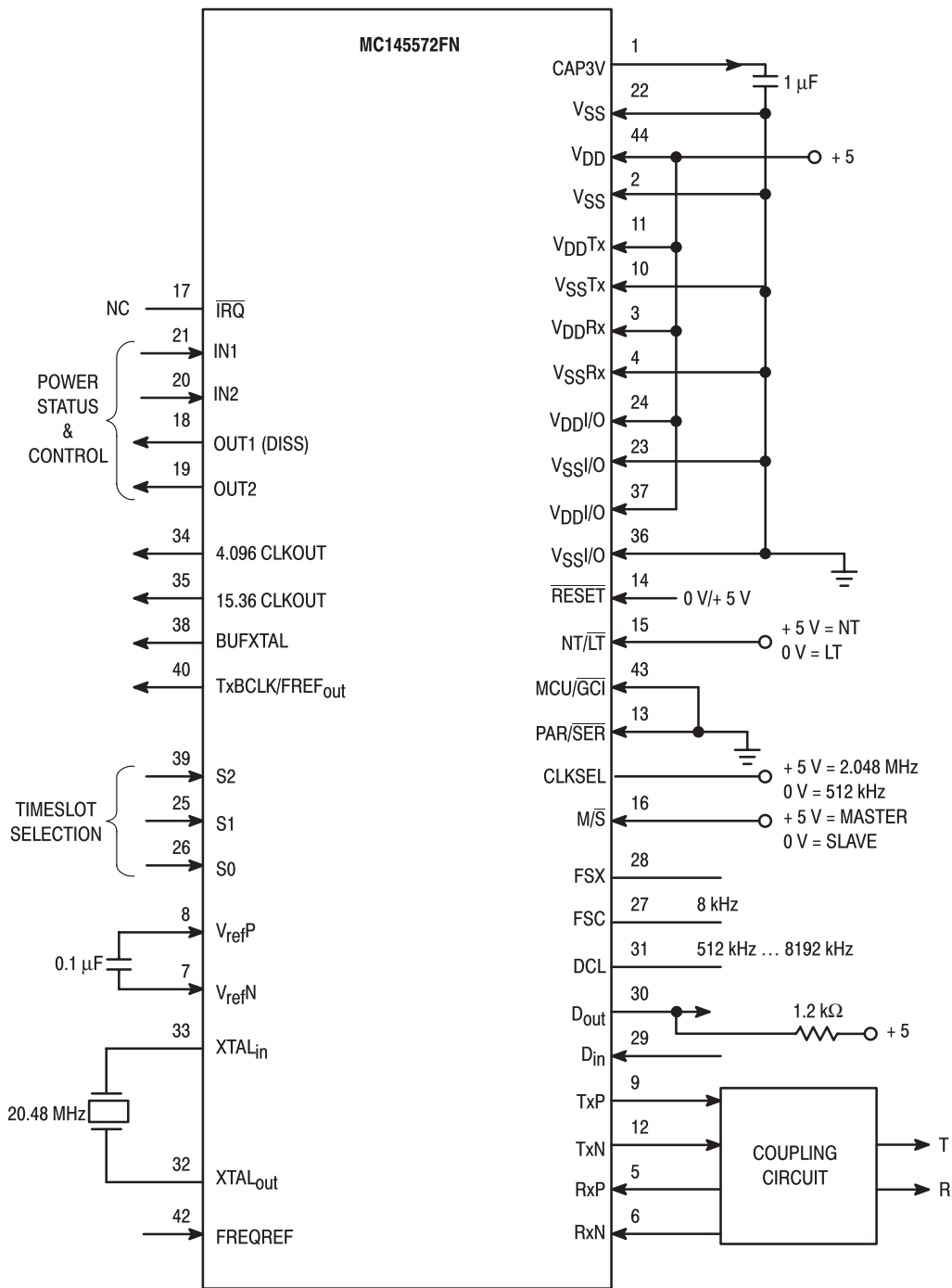
Figure 8-1. MC145572 Configuration for GCI Operation
