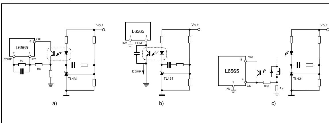
Figure 23. Secondary Feedback loop configurations
