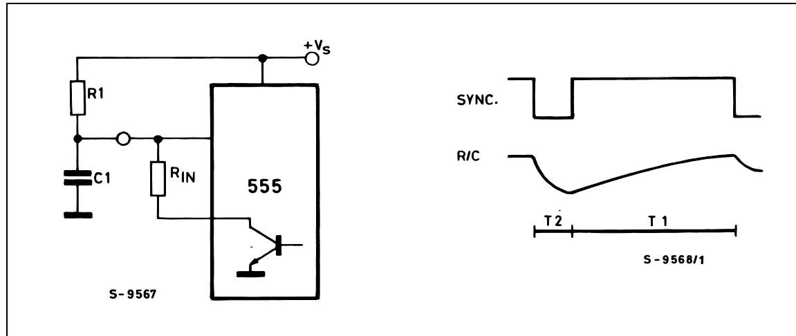
Figure 1 : Oscillator Circuit and Waveforms.
