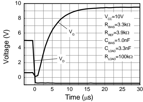
Switch-On Speed
