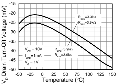
Turn-Off Voltage vs Temperature
