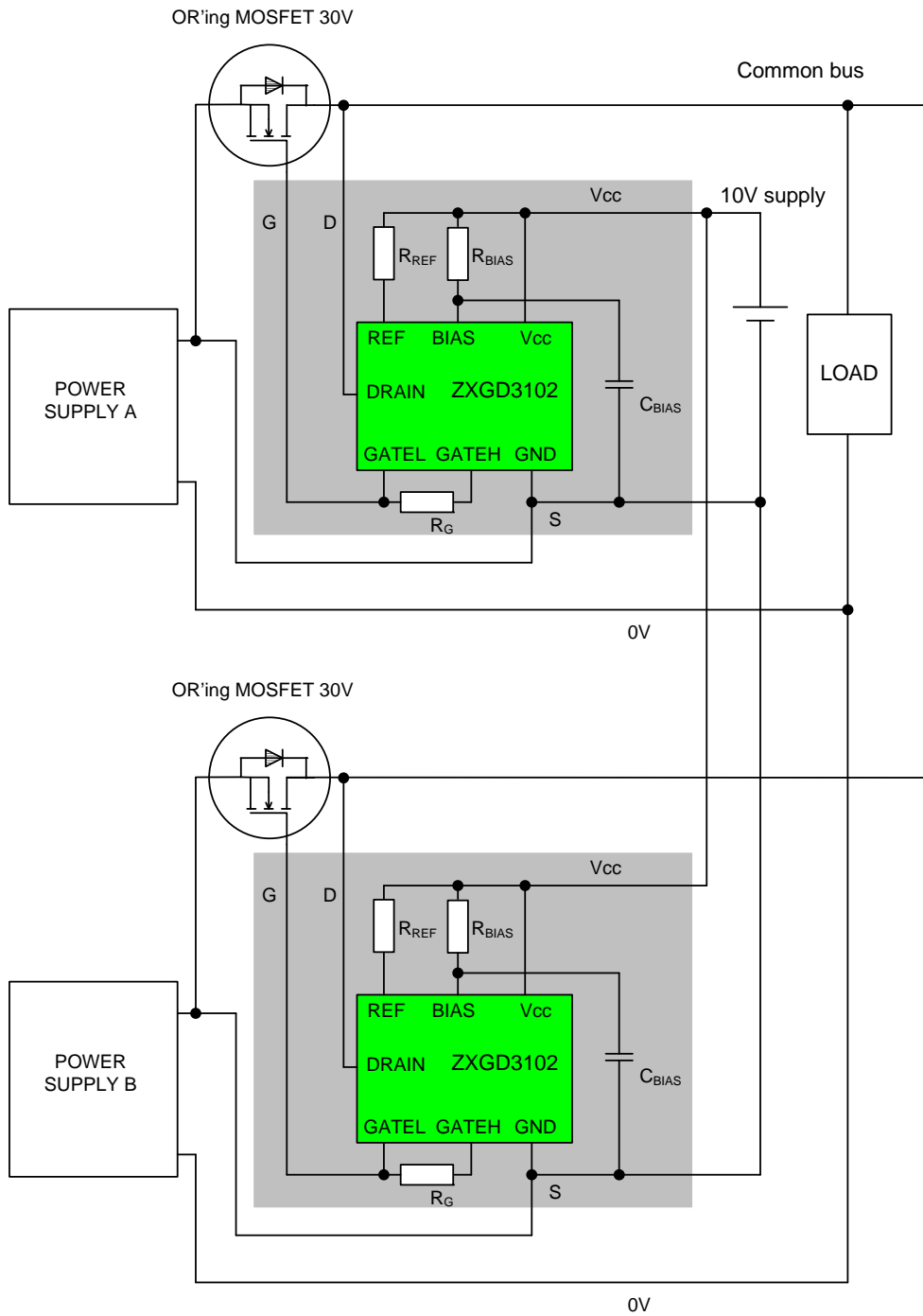
Figure 3: Positive rail power supply active OR'ing evaluation
