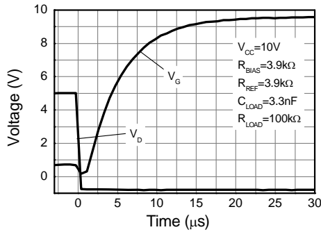
Switch-On Speed
