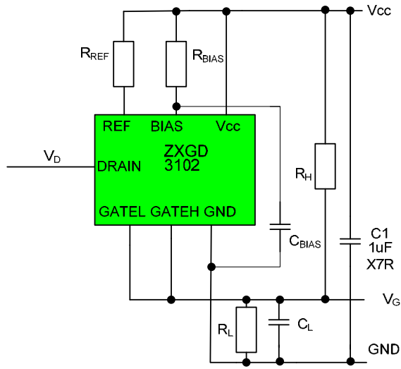
Figure 4: Test Circuit
