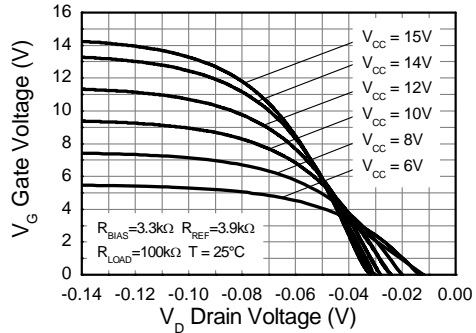
Transfer Characteristic
