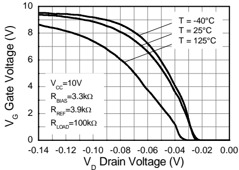
Transfer Characteristic
