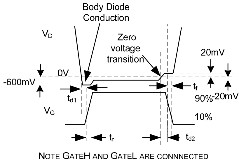
Figure 5: Timing Diagram
