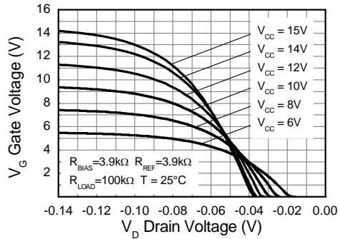
Transfer Characteristic
