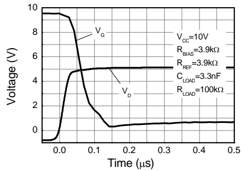
Switch-Off Speed
