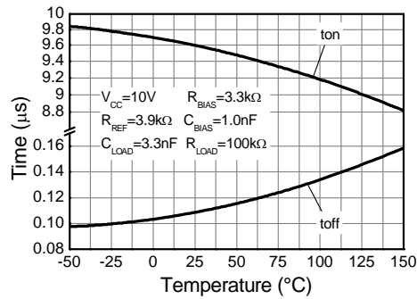
Speed vs Temperature
