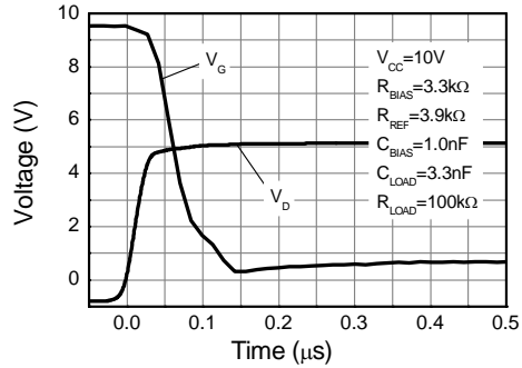
Switch-Off Speed
