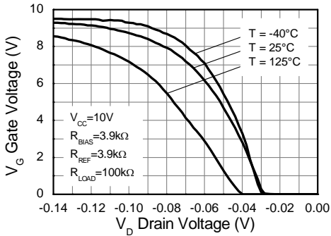
Transfer Characteristic
