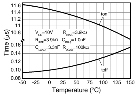
Speed vs Temperature
