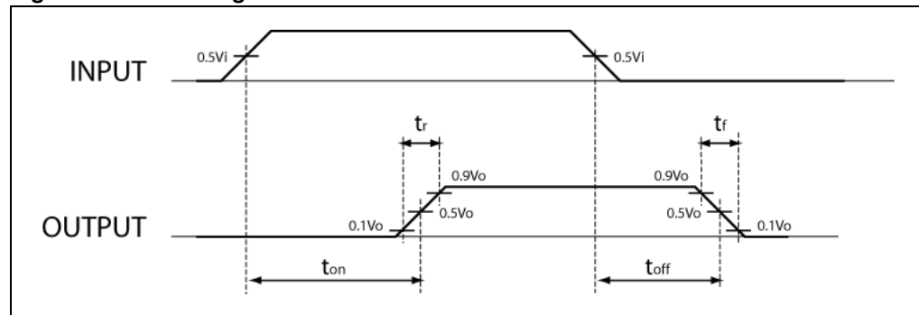
Figure 4. Switching times
