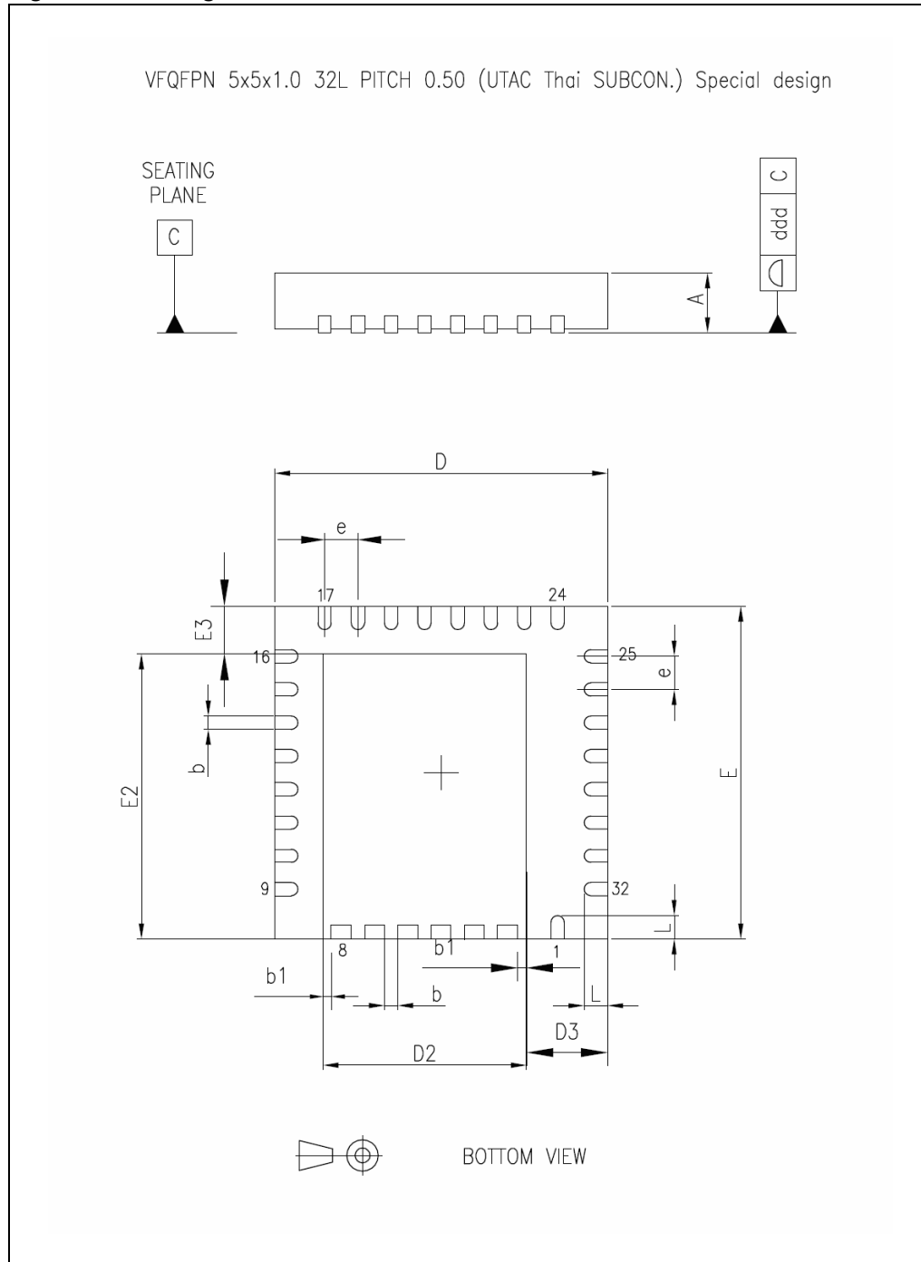
Figure 5. Package dimensions
