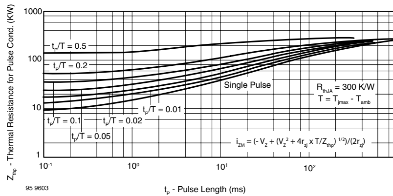
Figure 10. Thermal Response
