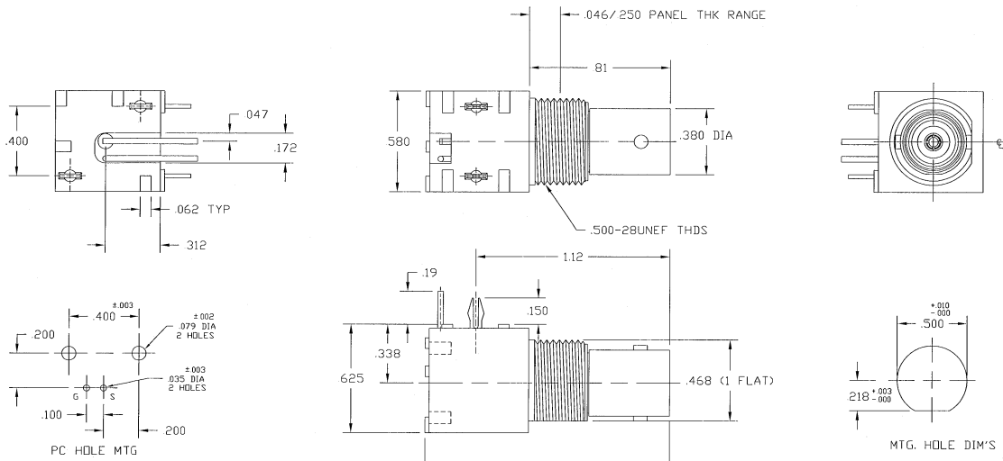
CUSTOMER OUTLINE DRAWING
