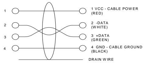
WIRING DIAGRAM
