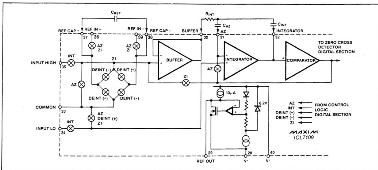
Figure 2. Analog Section
