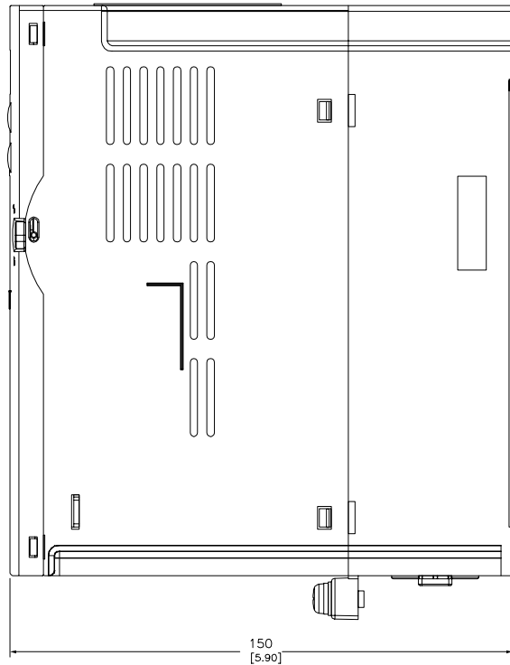
RIGHT VIEW
