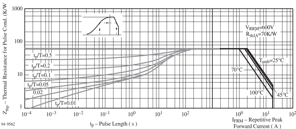
Figure 7. Thermal Response
