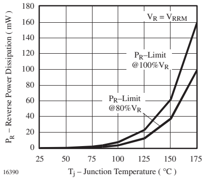
Figure 5. Max. Reverse Power Dissipation vs. Junction Temperature
