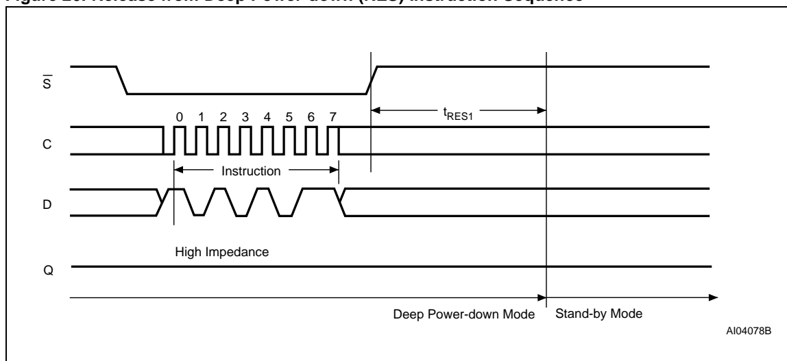
Figure 20. Release from Deep Power-down (RES) Instruction Sequence
