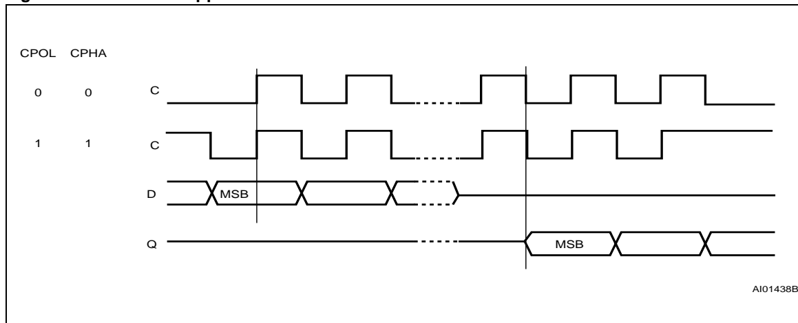
Figure 6. SPI Modes Supported
