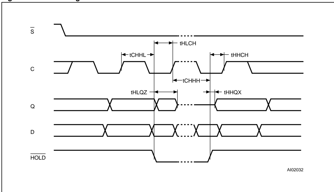
Figure 25. Hold Timing
