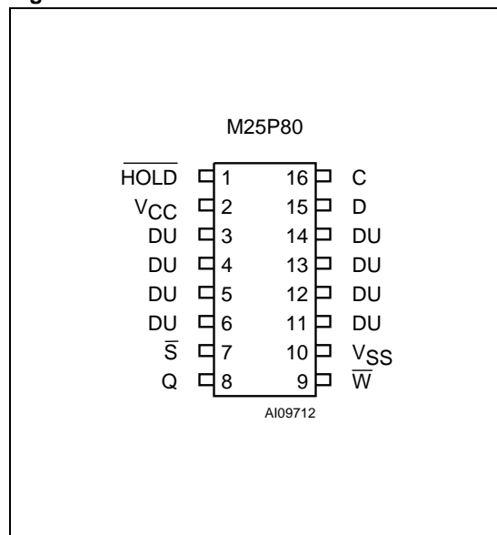
Figure 4. SO16 Connections
