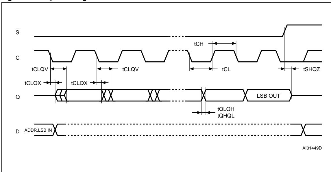
Figure 26. Output Timing
