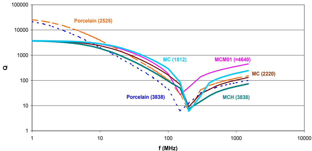
Q vs. Frequency 470 pF @ 25 °C
