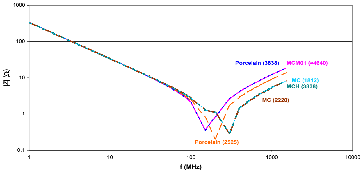
Impedance |Z| vs. Frequency for 470 pF @ 25 °C
