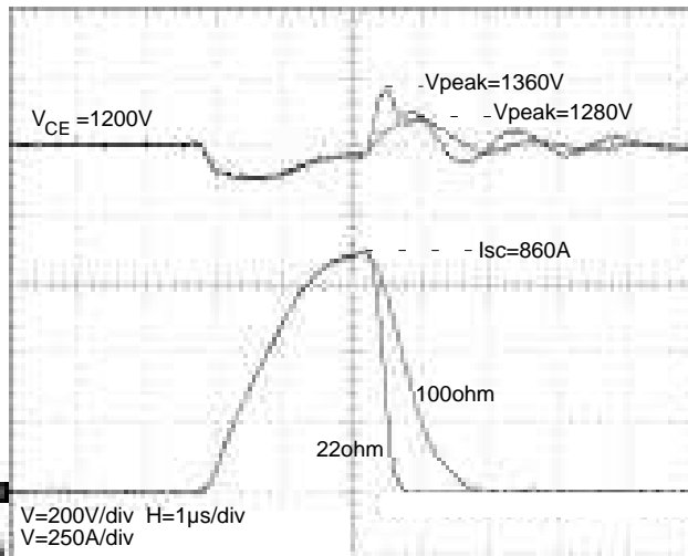
Fig.13 Effect of R_{\text{goff-SC}} in short - circuit
