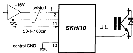
Fig.4b Connecting the SKHI10 with long cable
