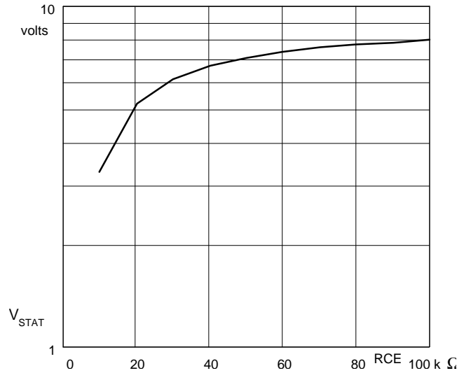
Fig.7b V_{CEstat} as function of R_{CE}
