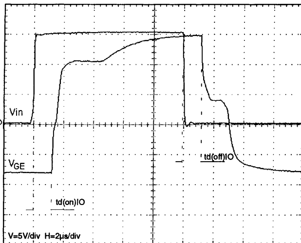
Fig. 10 Input and output voltage propagation time
