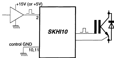
Fig.4a Connecting the SKHI10 with short cable
