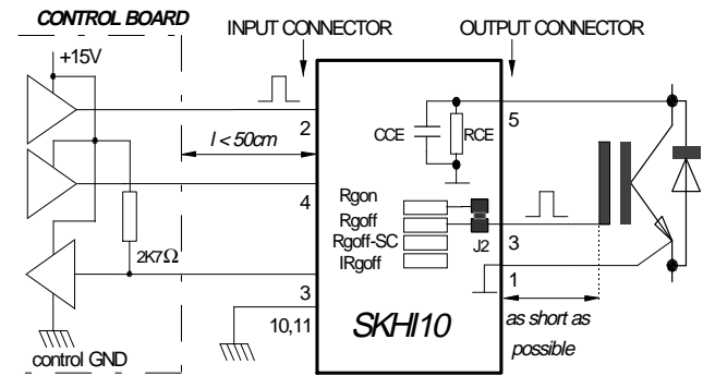
Fig. 8 Preferred standard circuit
