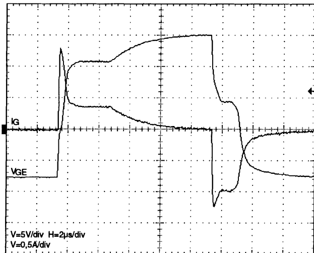
Fig. 11 Output voltage ( V_{GE} ) and output current ( I_G )
