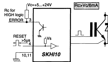
Fig.5 Driver status information ERROR, and RESET
