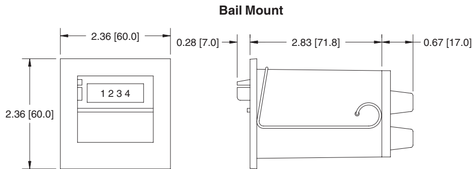
Panel cutout: 2.17" x 2.17" [55.1 x 55.1]
