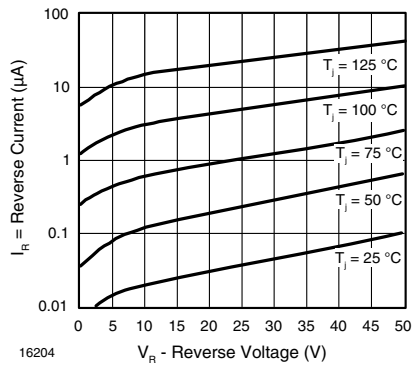
Figure 1. Reverse Current vs. Reverse Voltage
