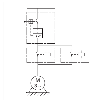
Figure 131. XTFR Combination Motor Controller
