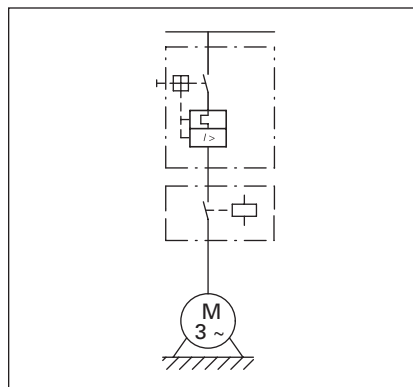
Figure 130. XTFC Combination Motor Controller
