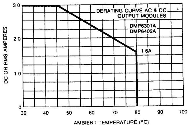
Figure 1. Maximum Output Current vs Ambient Temperature
