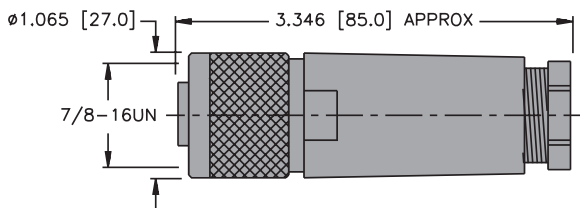
Female Connector
