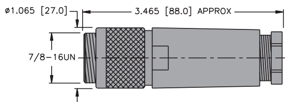
Male Connector
