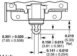
Swivel Link
