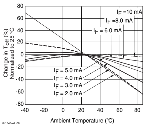
Figure 8. Turn-off Time vs. Temperature
