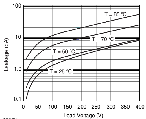
Figure 6. Leakage Current vs. Applied Voltage
