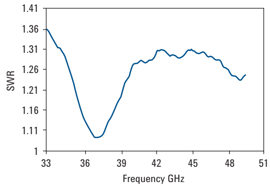
Typical SWR, 33 to 50 GHz ( 25\text{ }^{\circ}\text{C} \pm 10\text{ }^{\circ}\text{C} ) for N8486AQ power sensor
