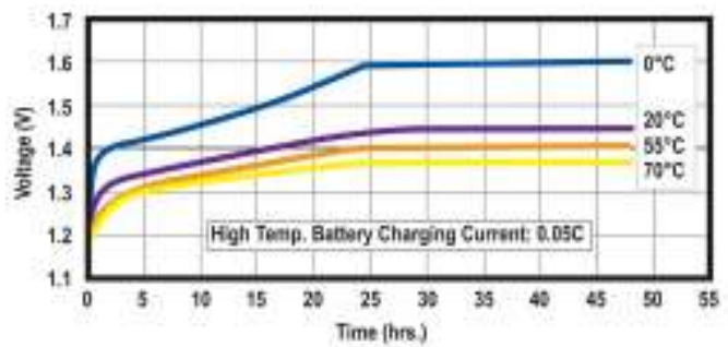
Trickle Charge
